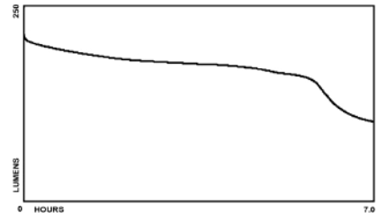
XPR-5568 PERFORMANCE CURVE
