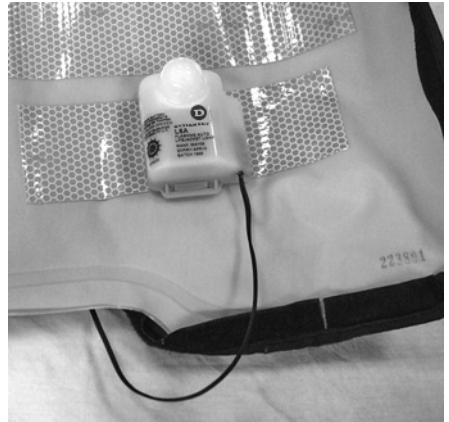
Example of L6A light fitted to jacket
